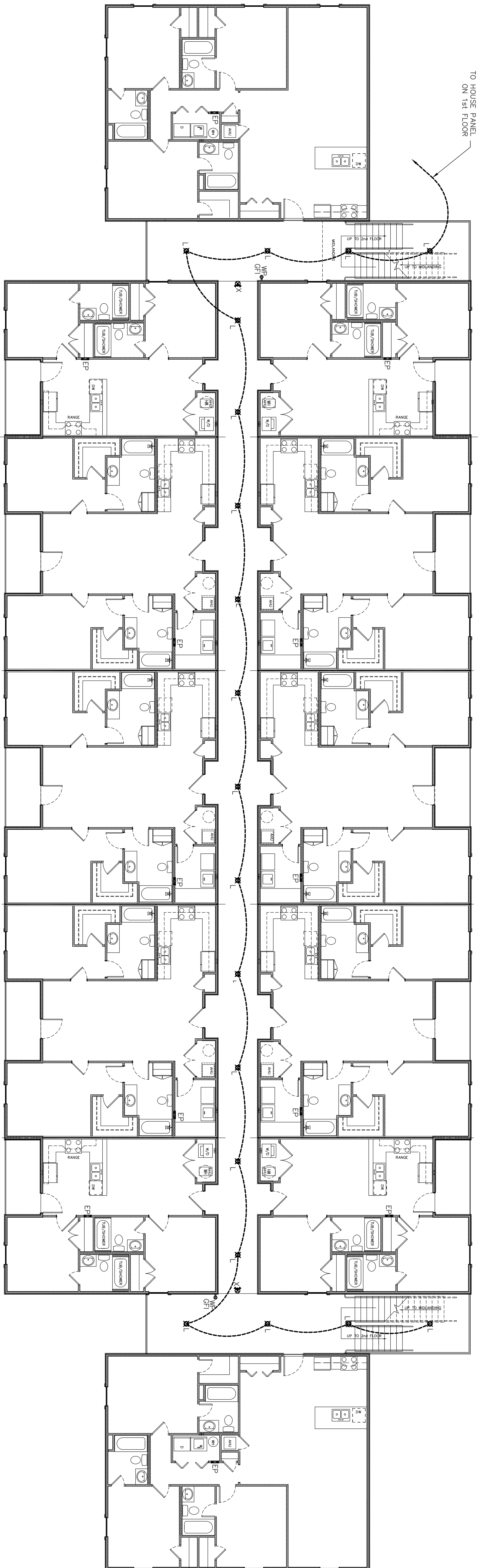
Electrical Plan - Building 'A' 2nd & 3rd Floor Scale: 1/8" = 1'-0"
