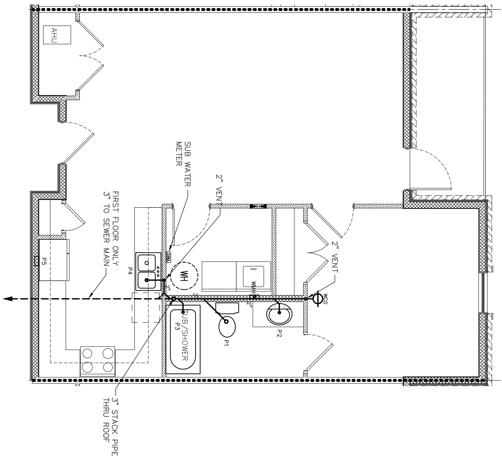
Plumbing Plan Typical 1-Bedroom Units - Bldg. "C" - 1st, 2nd & 3rd Floors Scale: 1/4" = 1'-0"
