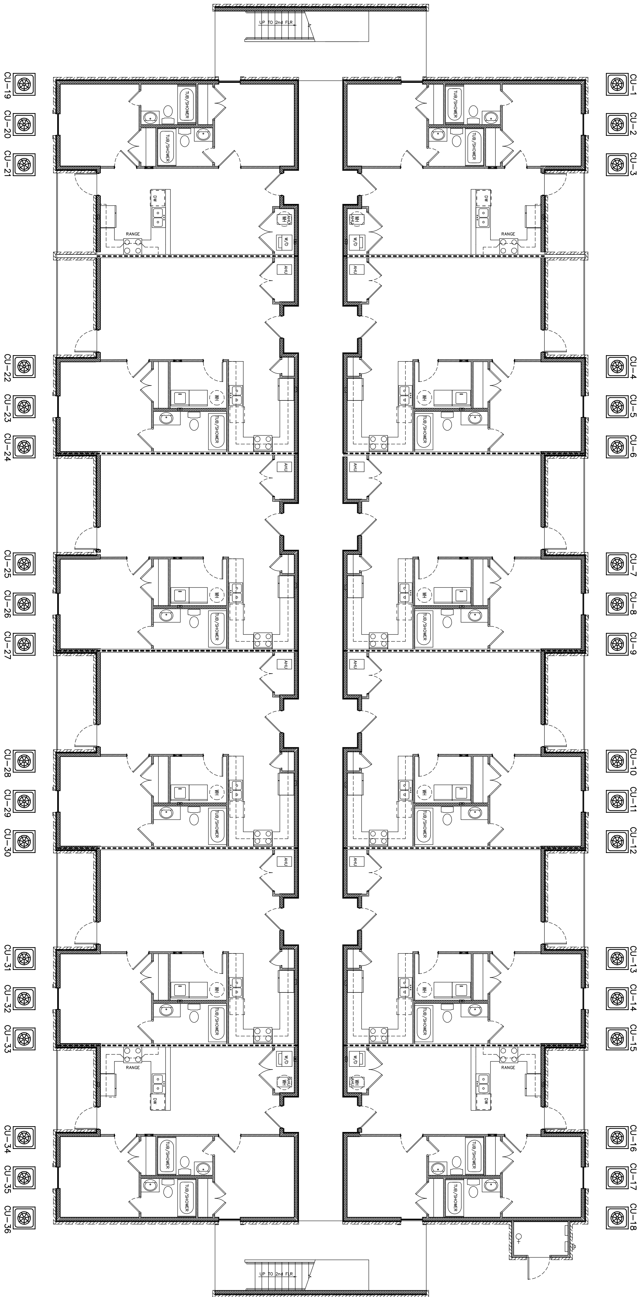
HVAC Plan - Building 'C' 1st Floor Scale: 1/8" = 1'-0"
